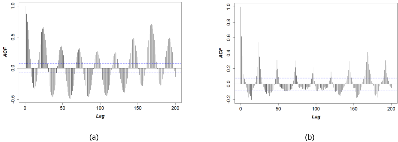
Figure 6 : daily electric energy consumption autocorrelations with a time lag ranging from one hour to 192 hours (8 days) for B1 (a) and B2 (b). Used data were measured from 01/09/2017 to 02/05/2017.
