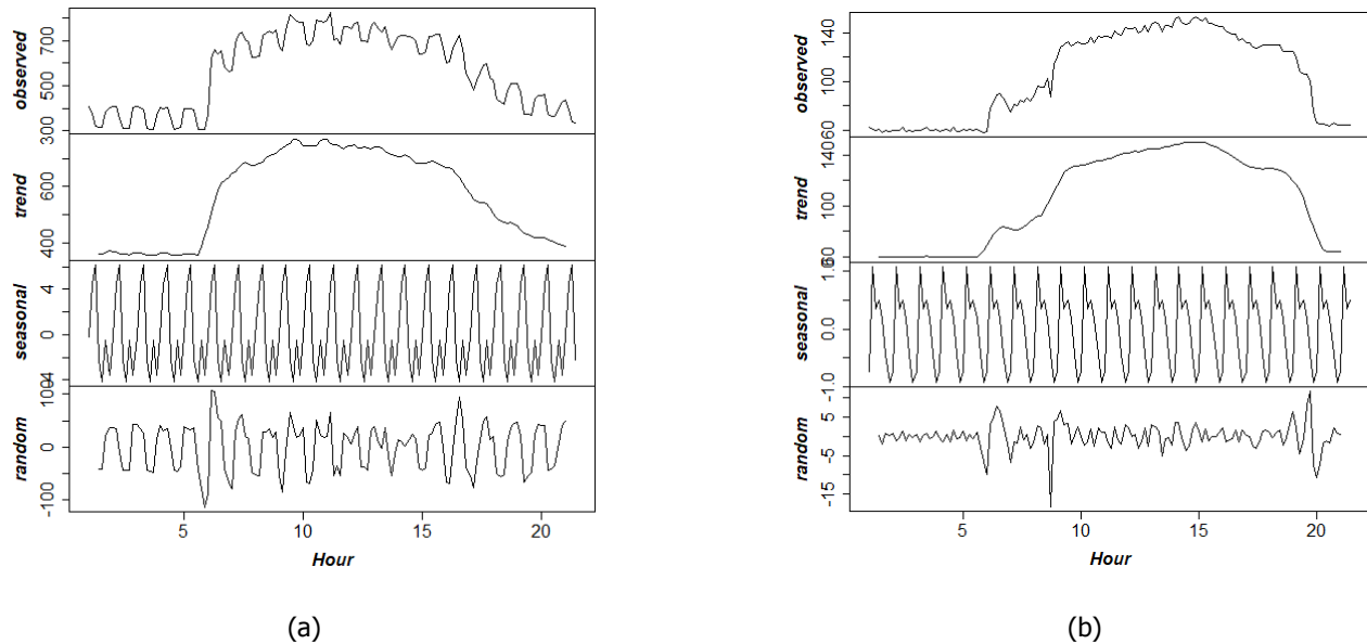
Figure 7 : Times series decomposition analysis of the electric energy consumption for B1 (a) & B2 (b), with a 10-minute time-step, the day of March 9 th , 2017.
