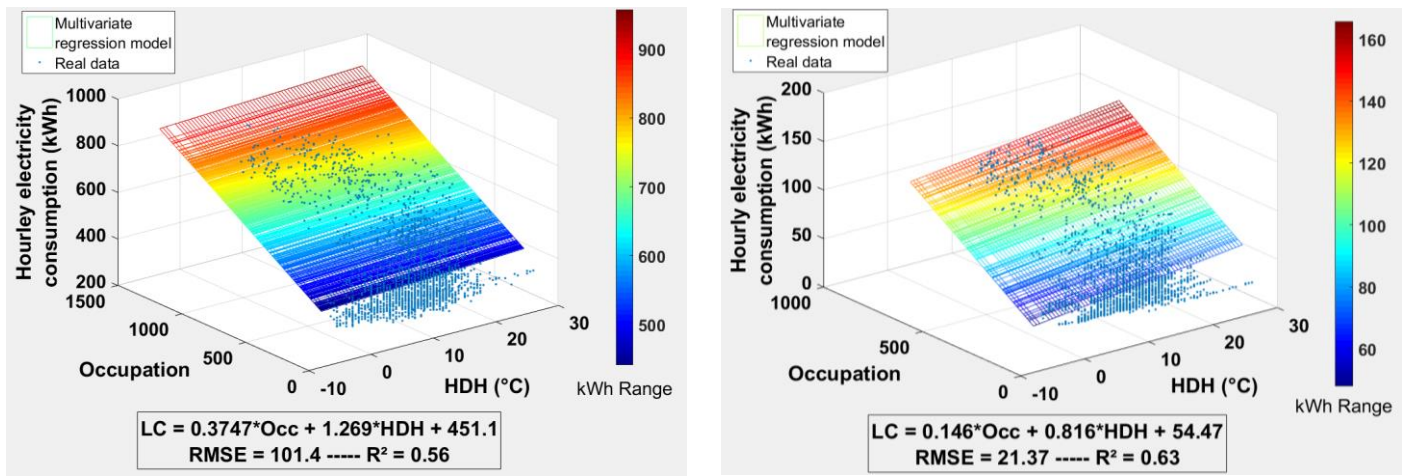
Figure 5 : Multi-variate regression of the electric energy consumption for B1 and B2 between 01/01/2017 to 04/27/2017.
