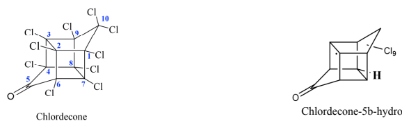
Figure 1. Chlordecone and chlordecone-5b-hydro structures (carbons numbered according to IUPAC)
