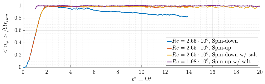
Figure 3: Influence of the bottom wall on the normalized velocity u_\varphi for spin-up and spin-down cases with and without a heavy salt water layer (Cam4, r/R = 0.77 ).
