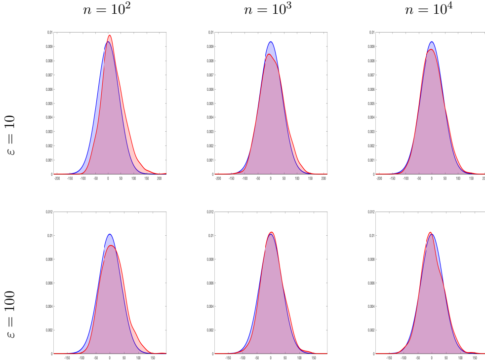
Figure 3: Case a \neq b with one sample. Illustration of the convergence in distribution of empirical Sinkhorn loss for a 20 \times 20 grid, \varepsilon = 10, 100 and n ranging from 10^2 to 10^4 . Densities in red (resp. light blue) represent the distribution of \sqrt{n}(\bar{W}_{p,\varepsilon}^p(\hat{a}_n, b) - \bar{W}_{p,\varepsilon}^p(a, b)) (resp. \langle G, \alpha_\varepsilon^{a,b} - 1/2(\alpha_\varepsilon^{a,a} + \beta_\varepsilon^{a,a}) \rangle ).
