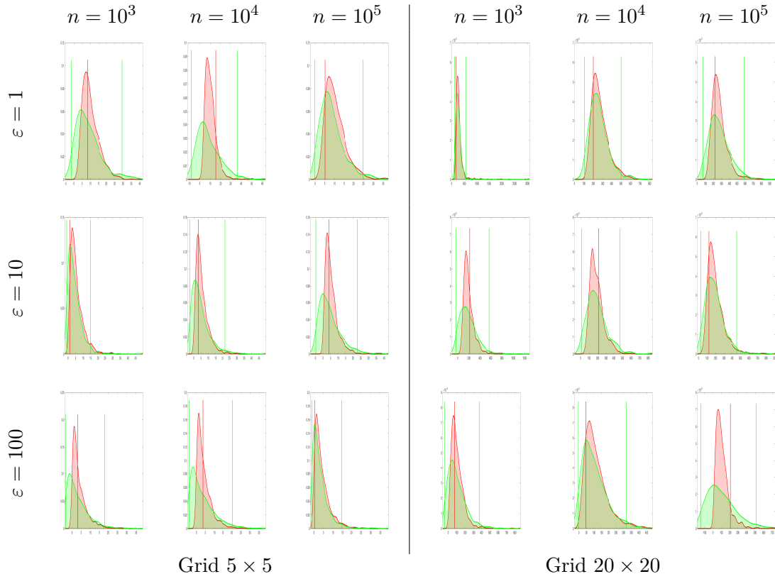
Figure 7: Case a = b with one sample. Illustration of the bootstrap with \varepsilon = 1, 10, 100 and two grids of size 5 \times 5 (left) and 20 \times 20 (right) to approximate the non-asymptotic distribution of the empirical Sinkhorn loss. Densities in red represent the distribution of n\bar{W}_{p,\varepsilon}^p(\hat{a}_n, a) . The green density represents the distribution of the random variable n(\bar{W}_{p,\varepsilon}^p(\hat{a}_n, a) - \bar{W}_{p,\varepsilon}^p(\hat{a}_n^*, a) - \langle \alpha^{\hat{a}_n, a}, \hat{a}_n^* - \hat{a}_n \rangle) in (3.1).
