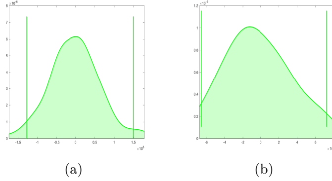
Figure 11: Testing equality of color distributions between Autumn and Winter for a grid of size 16^3 = 4096 . Green densities represent the distribution of the bootstrap statistics \rho_{n,m}^2(\overline{W}_{p,\varepsilon}^p(\hat{a}_n^*, \hat{w}_m^*) - \overline{W}_{p,\varepsilon}^p(\bar{a}_{20}, \bar{w}_{17}) - (\langle \alpha^{\bar{a}_{20}, \bar{w}_{17}}, \hat{a}_n^* - \bar{a}_{20} \rangle + \langle \beta^{\bar{a}_{20}, \bar{w}_{17}}, \hat{w}_m^* - \bar{w}_{17} \rangle)) (vertical bars represent a confidence interval of level 95%) for (a) \varepsilon = 10 and (b) \varepsilon = 100 . The value of \rho_{n,m}^2 \overline{W}_{p,\varepsilon}^p(\bar{a}_{20}, \bar{w}_{17}) is outside the support of the green density for each value of \varepsilon , and it is thus not represented.
