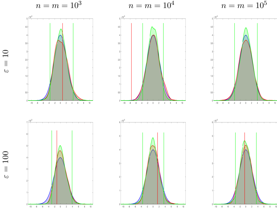
Figure 6: Case a \neq b with two samples. Illustration of the bootstrap with \varepsilon = 10 for the grid of size 5 \times 5 and \varepsilon = 100 for the grid 20 \times 20 to approximate the non-asymptotic distribution of empirical Sinkhorn divergences. Densities in red (resp. blue) represent the distribution of \rho_{n,m}(\bar{W}_{p,\varepsilon}^p(\hat{a}_n, \hat{b}_m) - \bar{W}_{p,\varepsilon}^p(a, b)) (resp. \sqrt{\gamma} \langle G, \alpha_\varepsilon^{a,b} - \frac{1}{2}(\alpha_\varepsilon^{a,a} + \beta_\varepsilon^{a,a}) \rangle + \sqrt{1-\gamma} \langle H, \beta_\varepsilon^{a,b} - \frac{1}{2}(\alpha_\varepsilon^{b,b} + \beta_\varepsilon^{b,b}) \rangle ). The green density is the distribution of the random variable \rho_{n,m}(\bar{W}_{p,\varepsilon}^p(\hat{a}_n^*, \hat{b}_m^*) - \bar{W}_{p,\varepsilon}^p(a, b)) in Theorem 3.2.
