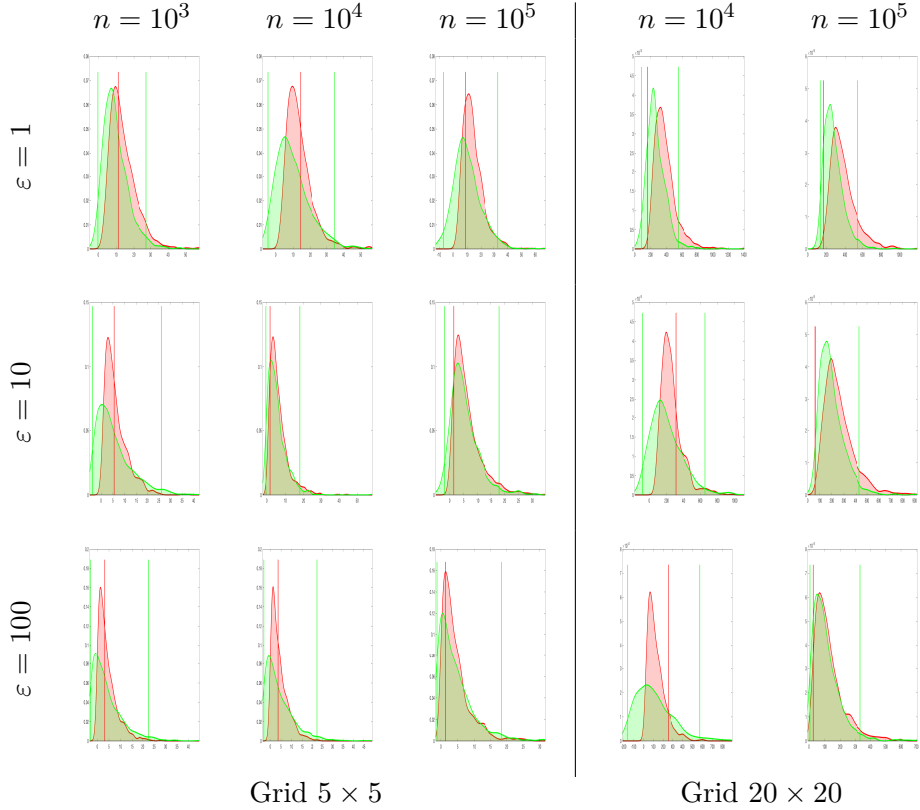
Figure 8: Case a = b with two samples. Illustration of the bootstrap with \varepsilon = 1, 10, 100 and two grids of size 5 \times 5 (left) and 20 \times 20 (right) to approximate the non-asymptotic distribution of the empirical Sinkhorn loss. Densities in red represent the distribution of \rho_{n,m}^2 \bar{W}_{p,\varepsilon}^p(\hat{a}_n, \hat{b}_m) . The green density represents the distribution of the random variable \rho_{n,m}^2 (\bar{W}_{p,\varepsilon}^p(\hat{a}_n^*, \hat{b}_m^*) - \bar{W}_{p,\varepsilon}^p(\hat{a}_n, \hat{b}_m) - \langle \alpha^{\hat{a}_n, \hat{b}_m}, \hat{a}_n^* - \hat{a}_n \rangle - \langle \beta^{\hat{a}_n, \hat{b}_m}, \hat{b}_m^* - \hat{b}_m \rangle) in (3.2).
