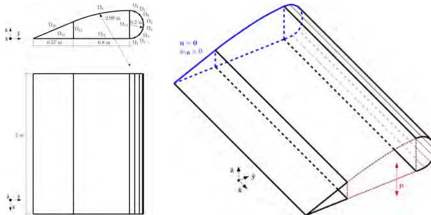
Fig. 7 Boundary conditions and geometric dimensions of a typical composite wing described in Section 4.1
