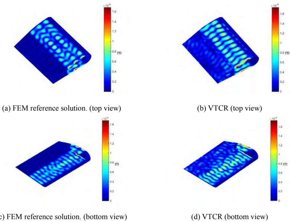
Fig. 8 Displacement magnitude portraits comparison at 500 Hz of the wing described in Section 4.1
