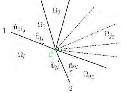
Fig. 4 n_c + 1 subdomains ( \Omega_i included) sharing the same corner C
