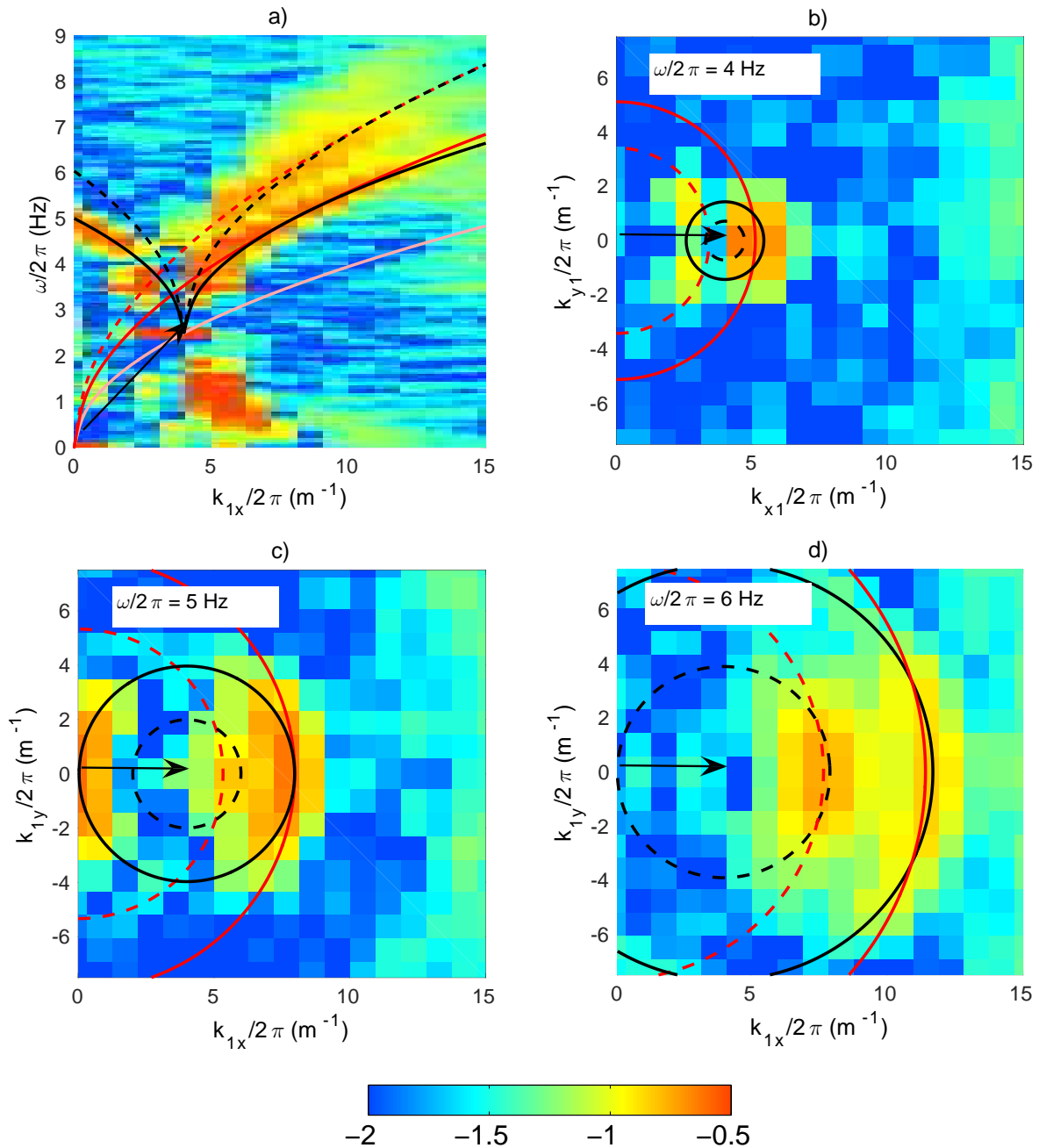
FIG. 10. 3D Bicoherence B_3^{k, \omega}(\mathbf{k}_2, \mathbf{k}_3, \omega_2, \omega_3) for a given wave (\mathbf{k}_2, \omega_2) (with |\mathbf{k}_2|/2\pi = 4 \text{ m}^{-1} ). In order to allow a direct comparison, the axes are the same than those of figure 8 and show \mathbf{k}_1 = \mathbf{k}_2 + \mathbf{k}_3 and \omega_1 = \omega_2 + \omega_3 . The x axis is given by the direction of \mathbf{k}_2 . The black arrows show the wave (\mathbf{k}_2, \omega_2) . (a) Cross-section in the plane (k_x, k_y = 0, \omega) . The red and black curves are similar to ones shown in fig 8. Exact resonances are at the intersection of a black curve and a red one. A high correlation intensity is observed in these regions, suggesting the occurrence of interaction between linear waves and harmonics. (b), (c) and (d) are three cross-sections in the planes corresponding to given values of \omega/2\pi = 4, 5 and 6 \text{ Hz} . An angular dispersion of the interactions of about 90^\circ is observed.
