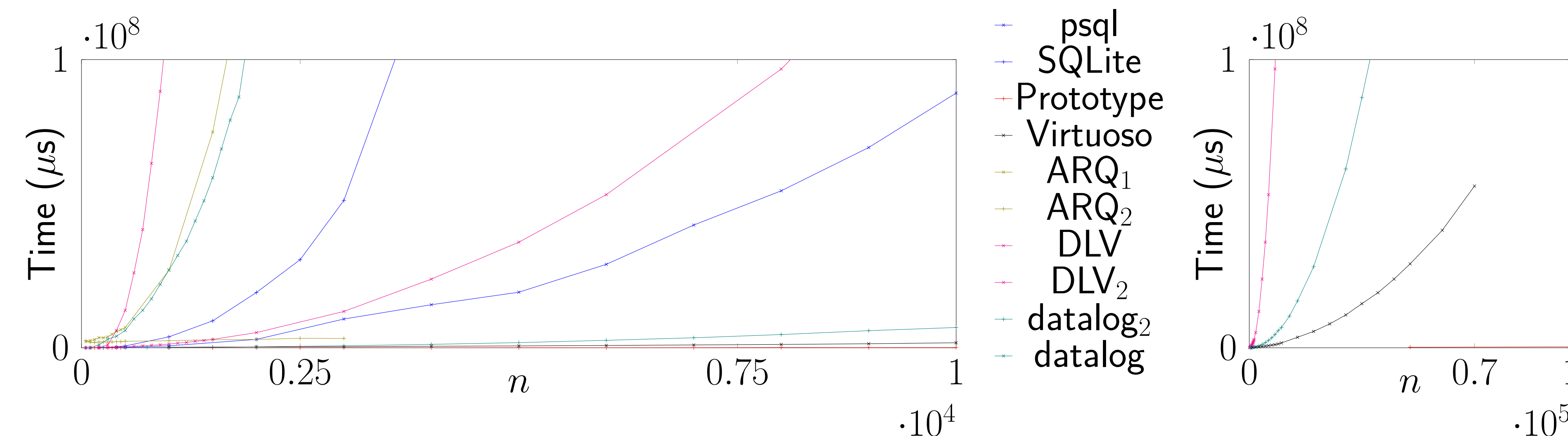
Figure 1: Evaluation time for the query \{?x \text{ knows } * ?y .?x \text{ named name}_{42}.\} on a graph of size n
