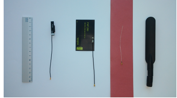
Figure 3. Different antennas. From left to right: PC81, FXP280, Laird and the dipole.
