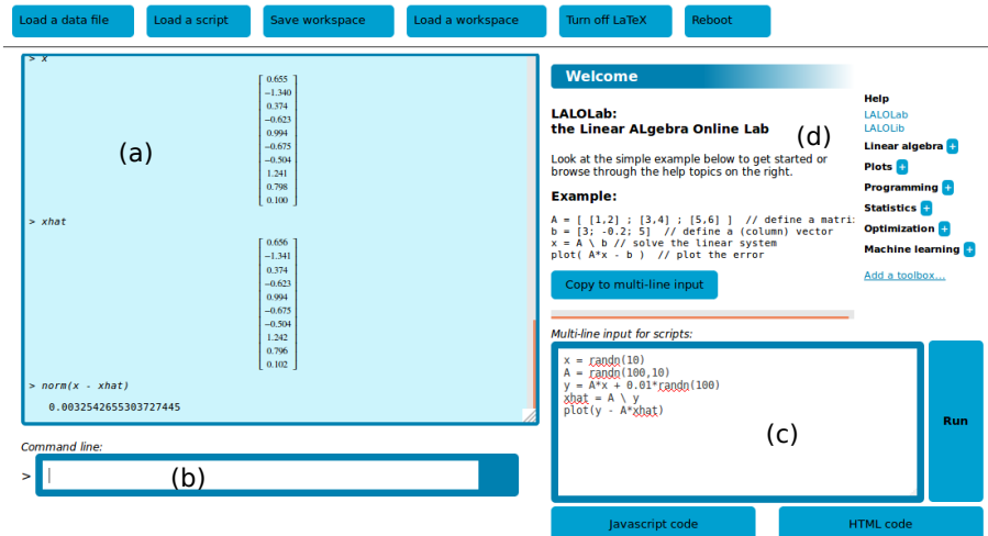
Figure 1: LALOLab web interface.
