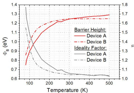
Fig. 5 – Barrier height and ideality factor extracted from I-V characteristics between 10µA and 100µA on both devices
