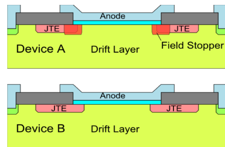
Fig. 1 – Schematic view of the structures of
