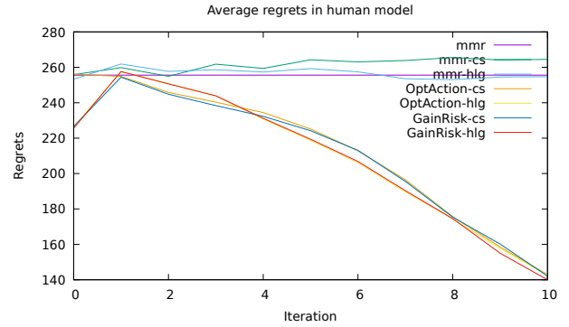
Figure 3: Average regret in user MDP (Generic).
