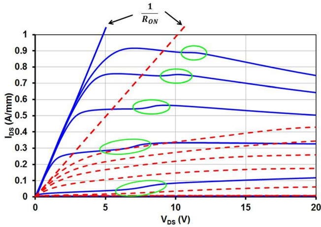
FIG. 1. I_{DS}(V_{DS}, V_{GS}) characteristics of AlInN/GaN HEMTs before (solid line) and after an on-state stress (dashed line). The drain-source voltage varies from 0 V up to 20 V and gate-source voltage increases from -6 V up to 1 V by steps of 1 V. All measurements were carried out in darkness in an enclosure. The ageing test has been done at V_{DS}=20 V and V_{GS}=0 V during 216 h in darkness.
