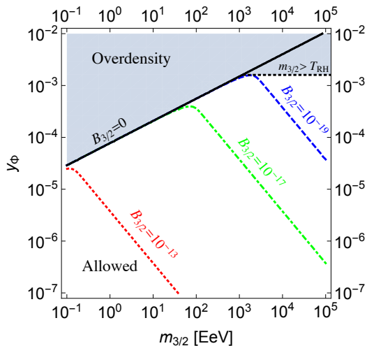
FIG. 1. Region of the parameter space allowed by PLANCK constraints [32] in the plane (m_{3/2}, y_{\phi}) for different values of the branching ratio B_{3/2} and m_{\phi} = 3 \times 10^{13} GeV (see the text for details).
