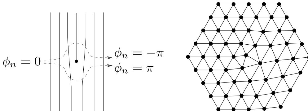
Figure 5: Dislocation in a charge density wave and a Wigner crystal. The stripes in the charge density wave are lines of constant phase Q(\hat{n} \cdot \vec{x} + \phi_n) , where Q\hat{n} is the CDW ordering wave vector.
