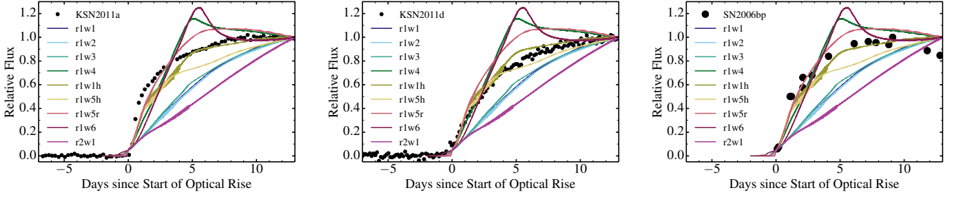
Fig. 12. Comparison between the optical flux (relative to the flux at 13 d) from our HERACLES simulations (we account for the flux between the Balmer and Paschen edges) and the observations of KSN 2011a (left), KSN 2011d (middle; Garnavich et al. 2016 ) and SN 2006bp (right; Quimby et al. 2007 ). The time origin is conveniently adjusted to correspond to the rise of the optical flux. A better match to the light curves is obtained for models with a dense/confined atmosphere/wind. None of our models match the fast rise of KSN 2011a.
