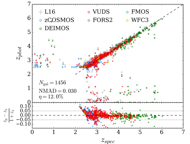
Fig. 4. Comparison between z_{\text{spec}} and z_{\text{phot}} , for spectroscopic galaxies (and stars) with [3.6] < 25 (empty circles). Only robust spectroscopic measurements ( \text{CL} > 95\% ) are plotted, and coloured according to their survey: zCOSMOS faint (Lilly et al., in preparation), VUDS (Le Fèvre et al. 2015), FMOS-COSMOS (Silverman et al. 2015), a survey with the FORS2 spectrograph at VLT (Comparat et al. 2015), a survey with DEIMOS at Keck II (Capak et al., in preparation), and grism spectroscopy from HST/WFC3 (Krogager et al. 2014). In the background we also show the comparison between z_{\text{spec}} and the original photometric redshifts of L16 (grey crosses). Upper panel: In addition to z_{\text{phot}} vs z_{\text{spec}} , in the bottom-left corner we report the number of objects considered in this test ( N_{\text{gal}} ), the \sigma_z error defined as the NMAD, and the fraction of catastrophic outliers ( \eta ). The dashed line is the z_{\text{phot}} = z_{\text{spec}} reference. Lower panel: Scatter of the z_{\text{phot}} - z_{\text{spec}} values, with the same colour code as in the upper panel. Horizontal lines mark differences (weighed by 1 + z_{\text{spec}} ) equal to \pm 0.05 (dotted lines) or null (dashed line).
