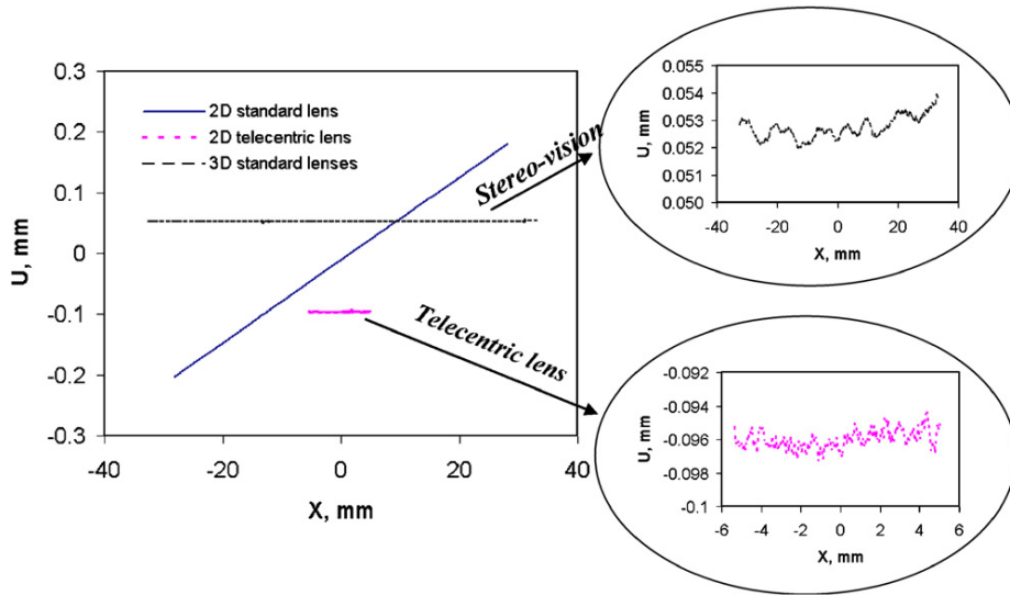
Fig. 7. Typical form of measured horizontal displacement, U(X, Y_s) (520 pixels), along line through image center for W = 5.5 mm using all three optical systems. Variability in the measurements is clearly visible in expanded views.
