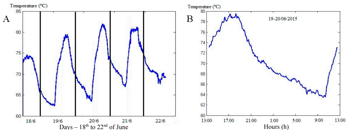
Figure 14. (A) Change in temperature over five days in the left gas spot of Figure 7C; (B) details of variation over 24 h (19/20 June 2015).
