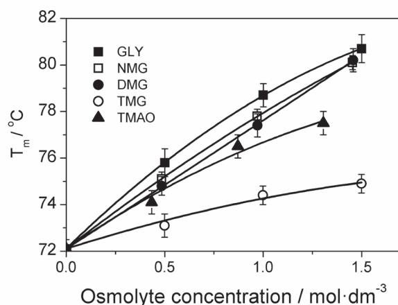
Figure 1. The dependencies of lysozyme's denaturation temperature (the maximum of the first derivative of CD-UV melting curves) versus osmolytes concentration.
