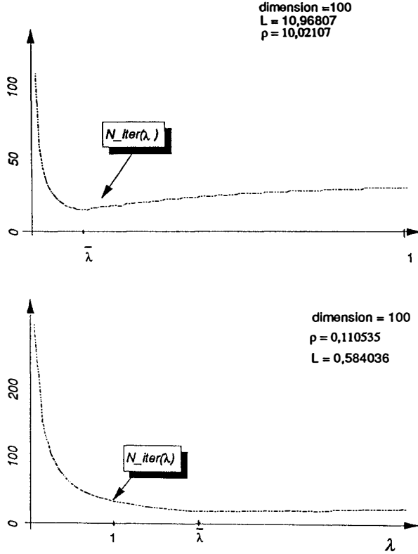
FIG. 2. Number of iterations for \text{dim}=100 .
