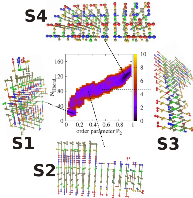
Figure 1: The free energy landscape (in k_B T^* ) of the A\beta_{37-42} 40-mers as a function of the order parameter P_2 and total number of inter-chain H-bonds at T^* = 0.19 (folding temperature of the monomer). Representative structures corresponding to the states S_i are shown. The color used for the amino acids is G + (red) - G (yellow) - V (grey) - V (grey) - I (green) - Ala - (blue).
