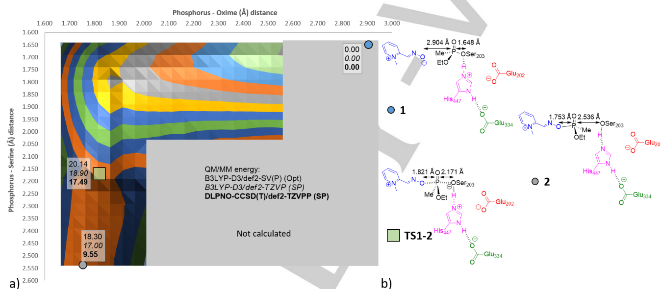
Figure 3. Reactivation of AChE with unprotonated Glu202 a) Potential energy surface as a function of the distance between the phosphorus and Ser203 and the distance between the phosphorus and 2-PAM. The position of the key geometries is highlighted with the energy in kcal.mol -1 b) Key geometries. Distances in Angström.
