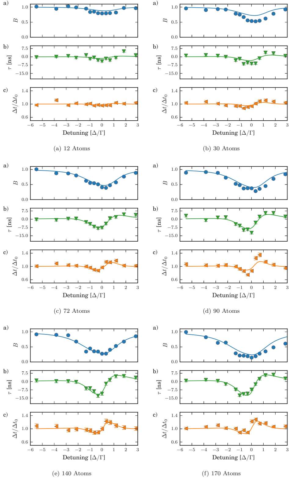
FIG. 5. For each group of figures corresponding to a given number of atoms: (a) Comparison between the amplitude B obtained by fitting the measured transmitted pulse (markers) and the one obtained from the fit of the reconstructed pulse (solid line). (b) Comparison between the delay \tau obtained by fitting the measured pulse (markers) and the one obtained from the reconstructed pulse (solid line). (c) Ratio between the temporal width \Delta t of the pulse after transmission and the width \Delta t_0 of the incident pulse measured in the absence of atoms. The markers are obtained from fits of the measured transmitted pulses. The solid lines are obtained from fits of the reconstructed pulses. Error bars are from the Gaussian fits to the data.
