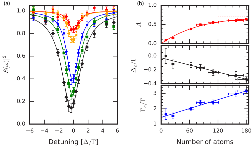
FIG. 4. (a) Measurements of |S(N, \Delta)|^2 deduced from transmission spectra measured in steady state for N = \{10, 25, 63, 83, 180\} (top to bottom). Error bars are rms statistical uncertainties. Solid lines: fits using the function of Eq. (1) (see the main text) with free parameters A(N) , \Delta_c(N) , and \Gamma_c(N) . (b) Fit results for the entire set of values of N used in this paper. Error bars are from the fits of the transmission spectra. Solid lines: fits of the data (see text). Dotted line: asymptotic value of A for N \gg 1 .
