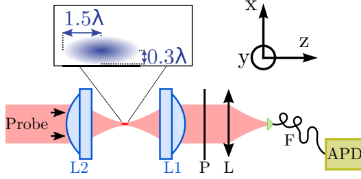
FIG. 1. Experimental setup. A microscopic cloud of ^{87}\text{Rb} atoms is illuminated by a linearly polarized probe laser focused down to a waist of w = 1.2 \mu\text{m} . P : polarization beam splitter, aligned at 45^\circ of the laser polarization. L : lens allowing the mode matching between the probe beam and the fiber mode in the absence of atoms. F : single-mode fiber. APD: avalanche photodiode.
