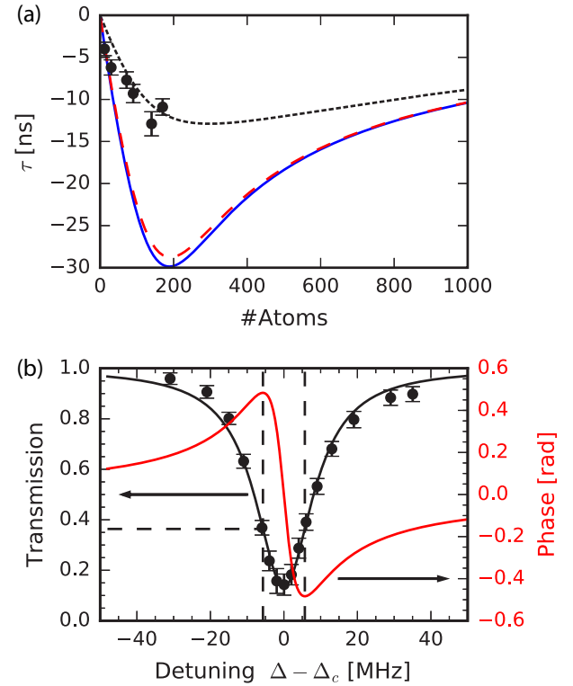
FIG. 3. (a) Largest group delay induced by the cold-atom cloud versus number of atoms. Dots: measured data. Dotted line: simulation based on Eq. (2) and using the measured transfer function S(\omega) [see Eq. (1)] and incoming pulse with a duration of \Delta t_0 = 25 ns (including the chirp). Solid line: prediction \tau_{\max}(N) based on Eq. (4). Dashed line: the same as the dotted line but taking a 200-ns-long pulse (without chirp). (b) Transfer function reconstructed from our measurements in steady state for N = 180 atoms. Black dots: measured data. Error bars: statistical uncertainties. Black line: fit by |S(\Delta - \Delta_c)|^2 . The horizontal axis is shifted by \Delta_c = -2 MHz. Red line: phase \phi = \arg[S] imprinted on the transmitted light by the cold-atom cloud. The dashed lines mark the extreme phase shifts and the associated transmission level.
