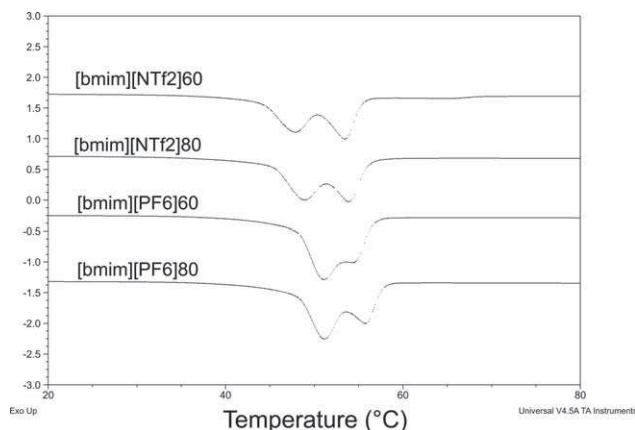
Figure 12. DSC thermograms of PCLs synthesized in ILs. Second scan of heating at a constant rate of 10^{\circ}\text{C min}^{-1} .
