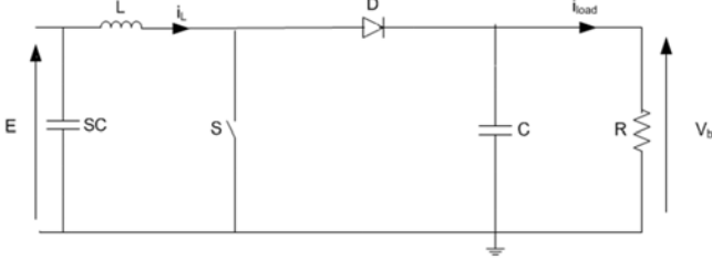
Figure 2 : Schematic of boost converter.
