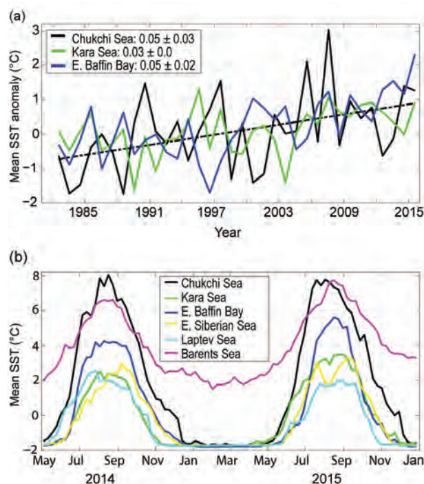
FIG. 5.8. (a) Time series of area-averaged SST anomalies (°C) for Aug of each year relative to the Aug mean for the period 1982–2010 for the Chukchi and Kara Seas and eastern Baffin Bay (see Fig. 5.7b). The dash-dotted black line shows the linear SST trend for the Chukchi Sea (the same warming trend as eastern Baffin Bay). Numbers in the legend correspond to linear trends (with 95% confidence intervals) in °C yr -1 . (b) SST (°C) in 2014–15 for each of the marginal seas, where the OISST V2 weekly product has been used in the calculation. For sea ice concentrations greater than 50%, the SST product uses a linear relationship with sea ice concentration to infer SST; variations in freezing temperature as a consequence of salinity variations imply that SSTs inferred from sea ice can be erroneously cool by as much as 0.2°C, with the highest errors in the Canadian sector (see Timmermans and Proshutinsky 2015).
