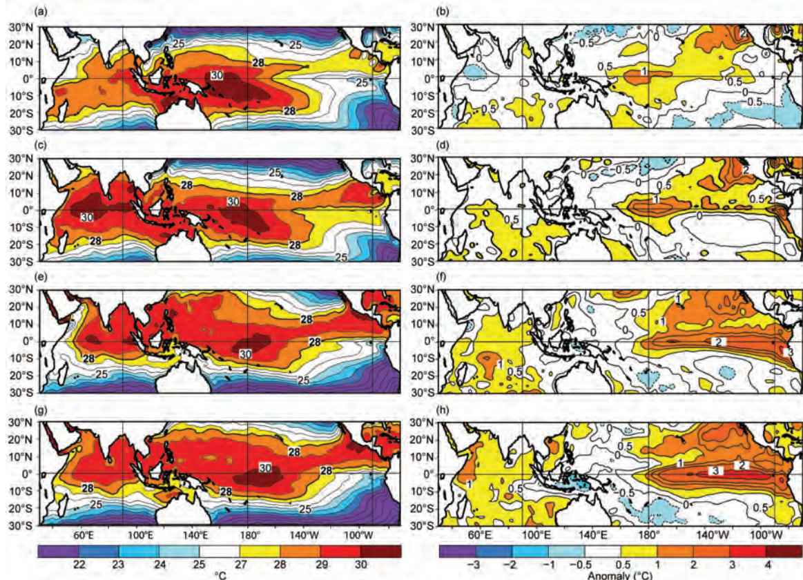
FIG. 4.2. Seasonal SST (left) and anomaly (right) for (a, b) DJF 2014/15, (c, d) MAM 2015, (e, f) JJA 2015, and (g, h) SON 2015. Contour interval for total SST is 1^{\circ}\text{C} . For anomalous SST, contour interval is 0.5^{\circ}\text{C} for anomalies between \pm 1^{\circ}\text{C} , and interval is 1^{\circ}\text{C} for anomalies > 1^{\circ}\text{C} or < -1^{\circ}\text{C} . Anomalies are departures from the 1981–2010 seasonal adjusted OI climatology (Smith and Reynolds 1998).
