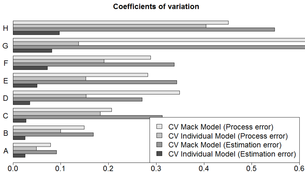
Figure 16: Coefficients of variation related to process and estimation errors, for both the Individual model and the Mack model.
