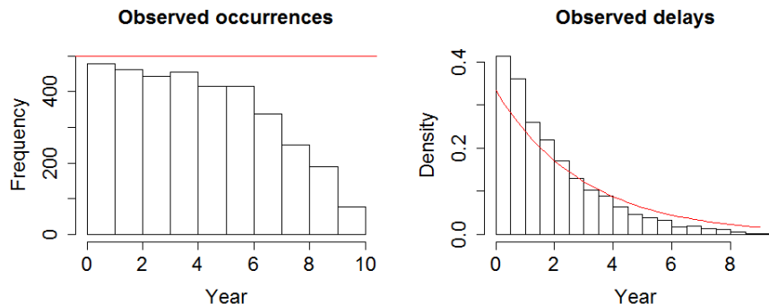
Figure 1: Distribution of observed occurrences (left) and delays (right) - each graph includes the underlying theoretical distribution in red.
