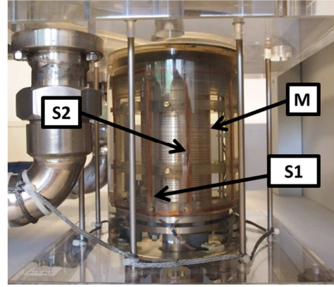
Fig. 1 – The fast-field cycling relaxometer and its compensation coils.
