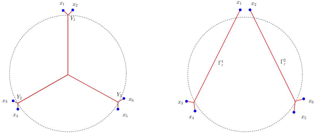
FIGURE 6. An example of a connected minimizer with six vortices of degree 1/3 .
