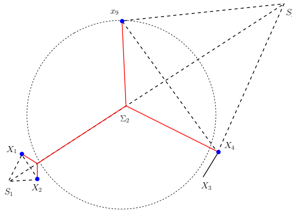
FIGURE 9. The set \Sigma_2 .
