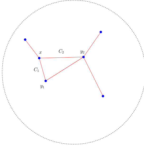
FIGURE 5. Construction of a competitor.
