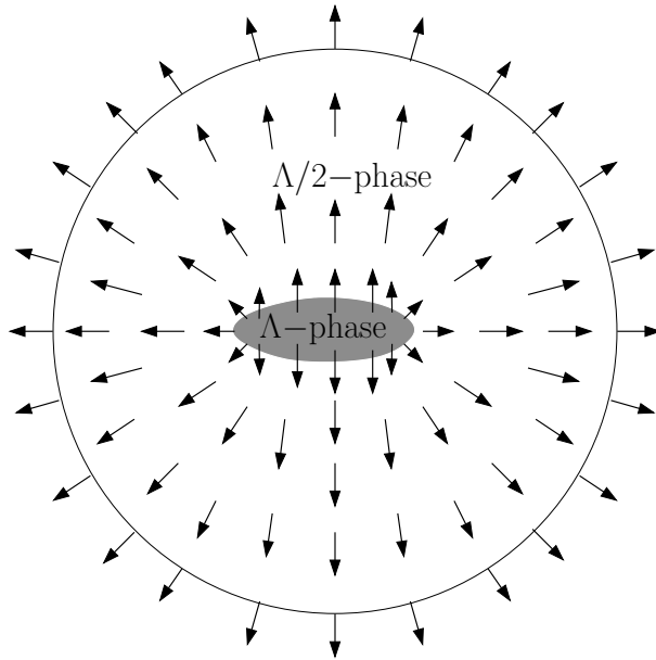
FIGURE 3. Creation of two vortices of degree 1/2 .
