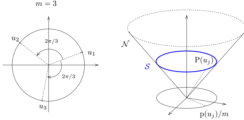
FIGURE 1. The cone \mathcal{N} and the projection P . P(u_1) = P(u_2) = P(u_3) .
