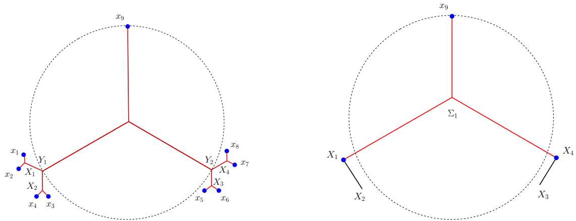
FIGURE 8. An example of a connected minimizer with nine vortices of degree 1/3 .
