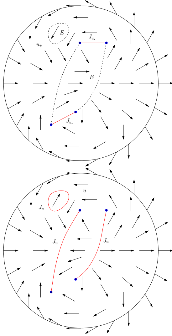
FIGURE 4. Cancellations in the case m = 2 ( E_1 = E , E_0 = \Omega \setminus E ).
