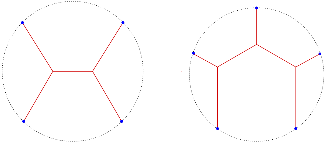
FIGURE 7. Minimizers of the Steiner problem for the vertices of the square on the left and of the regular pentagon on the right.
