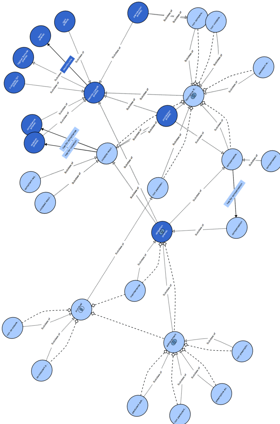
Figure 1. Overview of the NRV ontology and its core primitives
