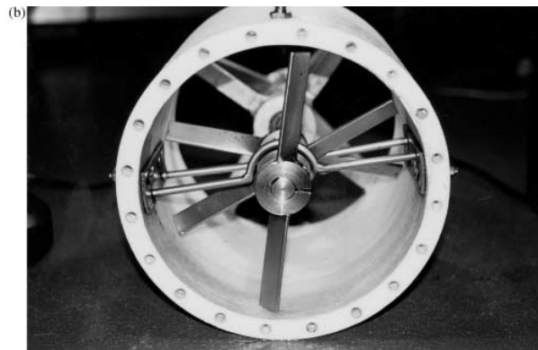
Figure 2. Detail of the heated wall of the dryer (a) and photograph of the blades and scrapers (b).
