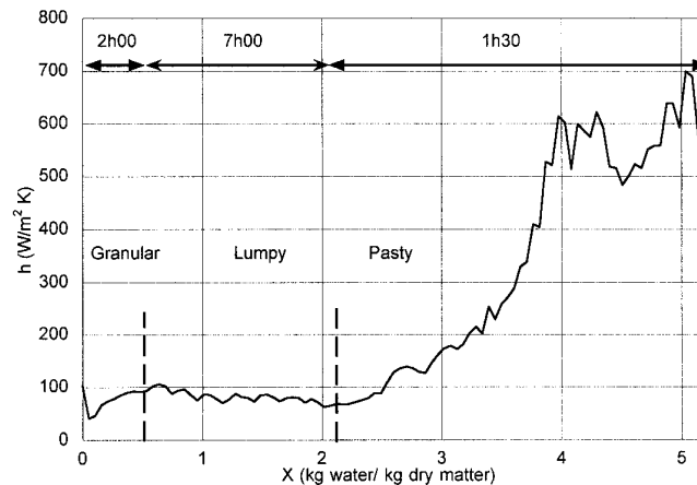
Figure 6. Evolution of the heat transfer coefficient between the heated wall and the sludge during drying for 120^\circ\text{C} regulation temperature, 20 rpm stirring speed, 2.2 kg initial mass, and 0.001 m distance between the first blade and the heated wall.
