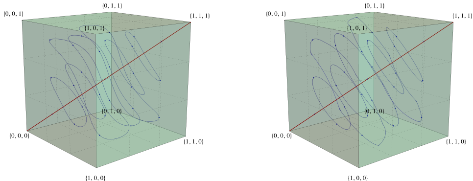
Figure 1. Evolution of the dynamics of FoReL in a 3-player zero-sum polymatrix game with entropic and Euclidean regularization (left and right respectively). The game considered is a graphical variant of Matching Pennies with three players. As can be seen, the trajectories of FoReL orbit the game’s line of Nash equilibria (dark red). The kinks observed in the Euclidean case occur when the support of the trajectory of play changes; by contrast, the multiplicative weights dynamics (left) are interior, so they do not exhibit such kinks.
