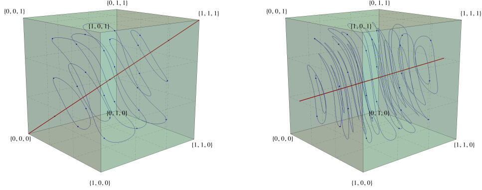
Figure 2. Evolution of the multiplicative weights dynamics (MW) in a 3-player zero-sum polymatrix game. In the left subfigure, each pair of players faces off in a game of standard (symmetric) Matching Pennies; in the right, the game on each pair is weighted by a different factor. In both cases, we plot the solution trajectories of (MW) for the same initial conditions. Even though the different weights change the trajectories of (MW) and the game’s equilibrium set, the cycling behavior of the dynamics remains unaffected.
