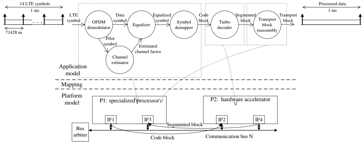
Fig. 21 Evaluated LTE communication receiver.
