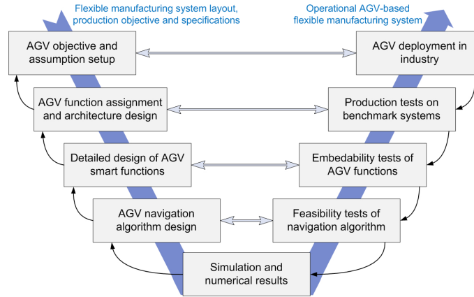
Fig. 2 Main steps of AGV design procedure until the deployment in industry
