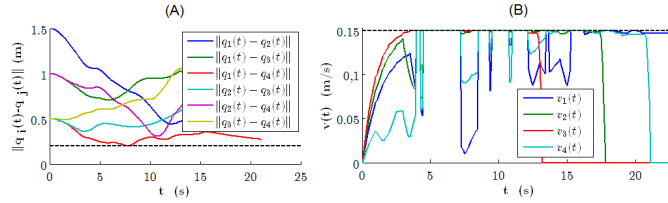
Fig. 5 Simulation of the illustrative example: AGV distances (A) and velocities (B)
