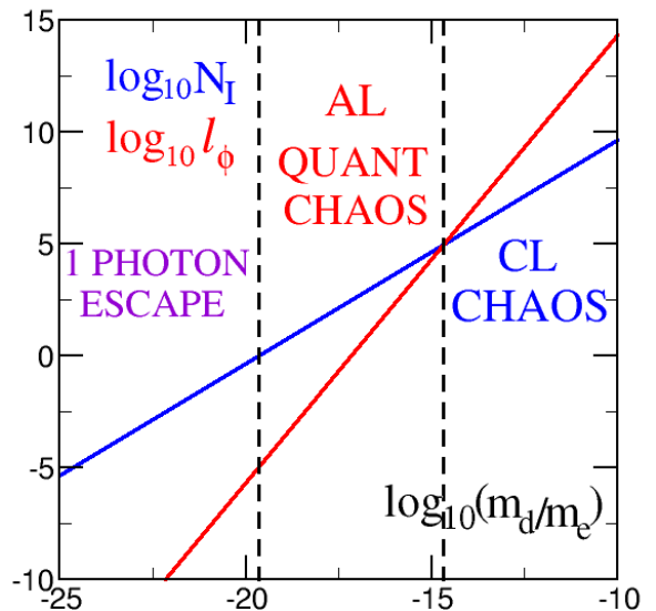
FIG. 1: (Color online) Dependence of number of photons N_I of Jupiter frequency required for ionization (escape) of DMP on its mass m_d rescaled by electron mass m_e (blue/black line), dependence of Anderson localization length of quantum chaos l_\phi on m_d/m_e (red/gray line); vertical dashed lines mark regimes of different ionization mechanisms of DMP: one photon escape (left), Anderson localization (middle), classical chaos with diffusive ionization (right); here initial DMP energy is E_d = -m_d v_J^2 / 2 .
