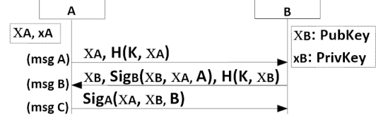
Figure 1: Authentication Procedure for a Wi-Fi based IoT
