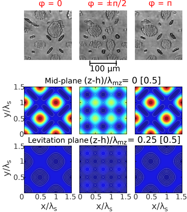
Fig. 10 Upper row: transmission microscope images of RBCs, excited at \omega = 37.1 MHz and 10 Vpp for all IDTs and for 3 different values of \varphi while keeping \phi_y^{\leftarrow} - \phi_y^{\rightarrow} and \phi_x^{\uparrow} - \phi_x^{\downarrow} constant (see also Movie S5). Middle and bottom rows: results of 3D numerical simulations of acoustic potentials in the horizontal planes (see supporting information SI2 ) at a height z/\lambda_{fz} = 0 [1/2] or in the levitation planes z/\lambda_{fz} = 1/4 [1/2] using f_1 = 0.11 39 and f_2 = 0.05 . The same colormap is used for both plots.
