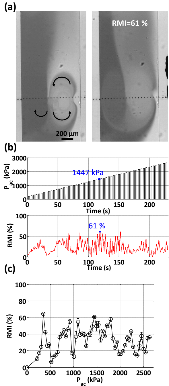
Fig. 6: Line shape: (a) Left: Vortices at the start of the P_{ac} = 1.45\ \text{MPa} mixing cycle, and right: maximum mixing during the cycle; (b) Acoustic pressure cycles and corresponding mixing efficiency; (c) Peak mixing efficiency during each pressure cycle against acoustic pressure.
