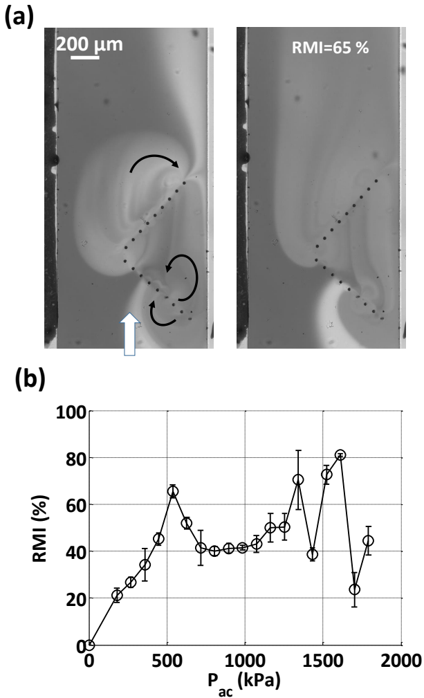
Fig. 16: (a) Modified left/right shape, P_{ac} = 537 kPa; (b) Mixing efficiency against acoustic pressure.
