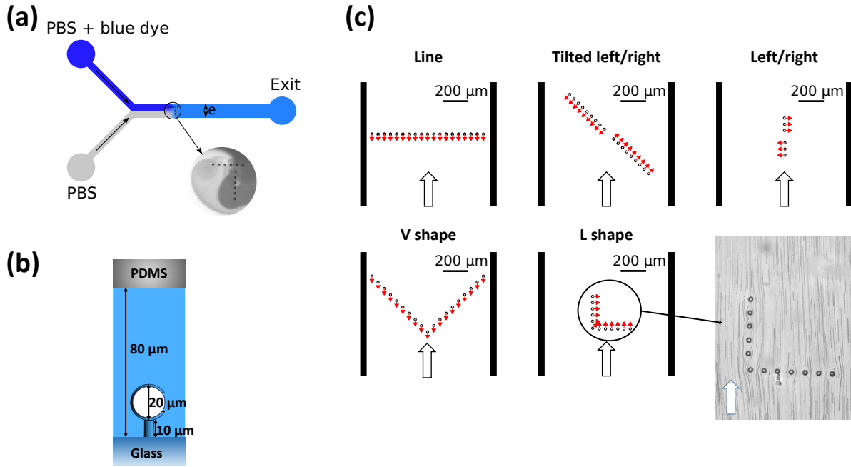
Fig. 4: (a) Y shaped microchannel used for mixing experiments. e = 1 mm. (b) Scale of the capsules used compared to the height of the channel. (c) Arrangements of capsules tested for mixing. Red arrows: direction of the opening. White arrows: input flow direction. Blown up L shape: experiment with a 1.2 mm/s input flow and no ultrasound.
