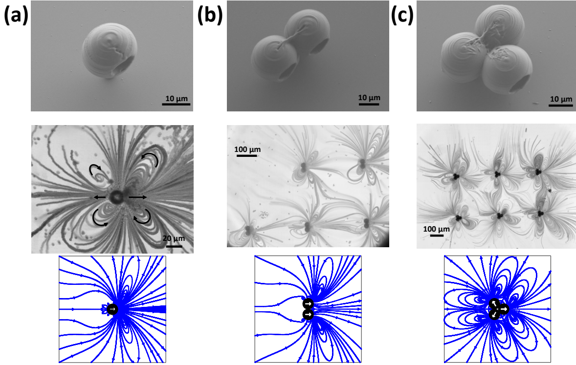
Fig. 2: Vortices generated by identical propulsors ( r = 9 \mu\text{m} , a = 5 \mu\text{m} , H = 10 \mu\text{m} ) arranged as: (a) Single propulsors; (b) Double propulsors; (c) Triple propulsors. Top line: SEM image, middle line: streamlines obtained by the superposition of tracer positions, bottom line: theoretical predictions of the streamlines.
