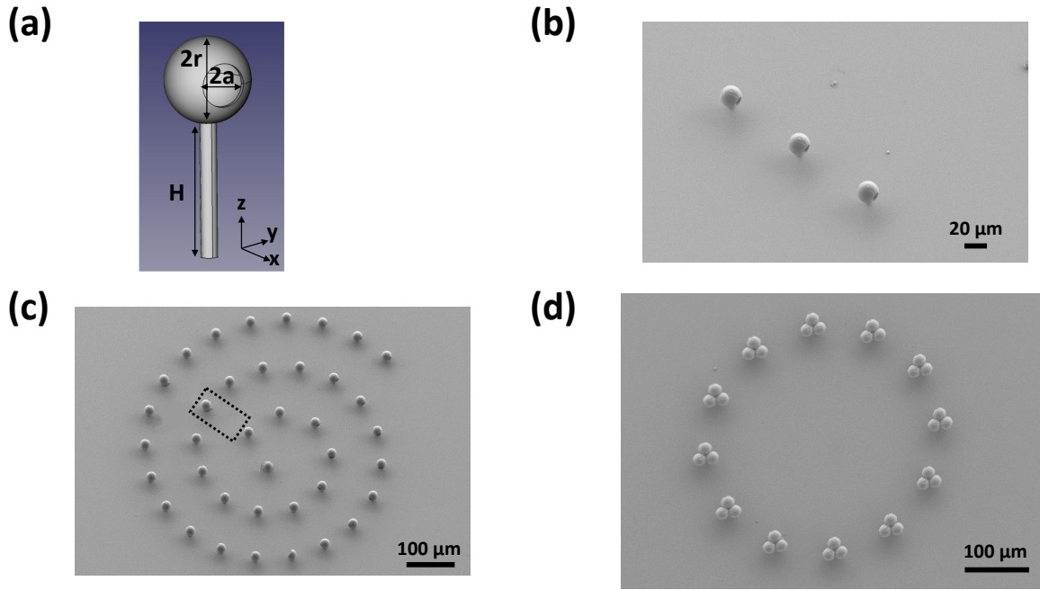
Fig. 1: (a) FreeCAD illustration and dimensions of the fabricated propulsors; (b) Scanning Electron Microscope (SEM) image of 3 propulsors; (c) Spiral of propulsors (a dust fiber has been edited out of the image next to an AMB, see dashed rectangle); (d) Triple propulsors arrange in a circle pattern.
