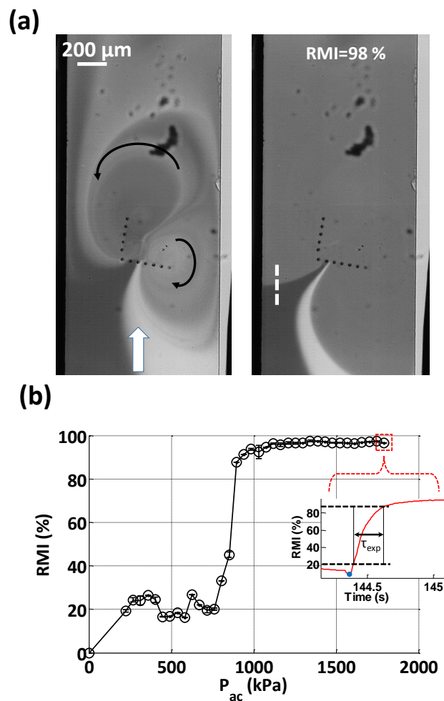
Fig. 13: (a) L shape in an e = 1 mm microchannel, P_{ac} = 1.34 MPa (dashed white line: segment taken to calculate the mixing time with ref. 4 ); (b) Mixing efficiency against acoustic pressure. Insert: RMI against total experiment time, with \tau_{exp} the time it takes to go from RMI = 20\% to RMI = 90\% . The blue circle represents the moment the ultrasound is turned back on.
