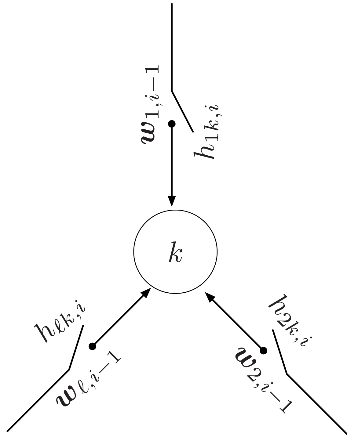
(b) Reduced-communication diffusion LMS
