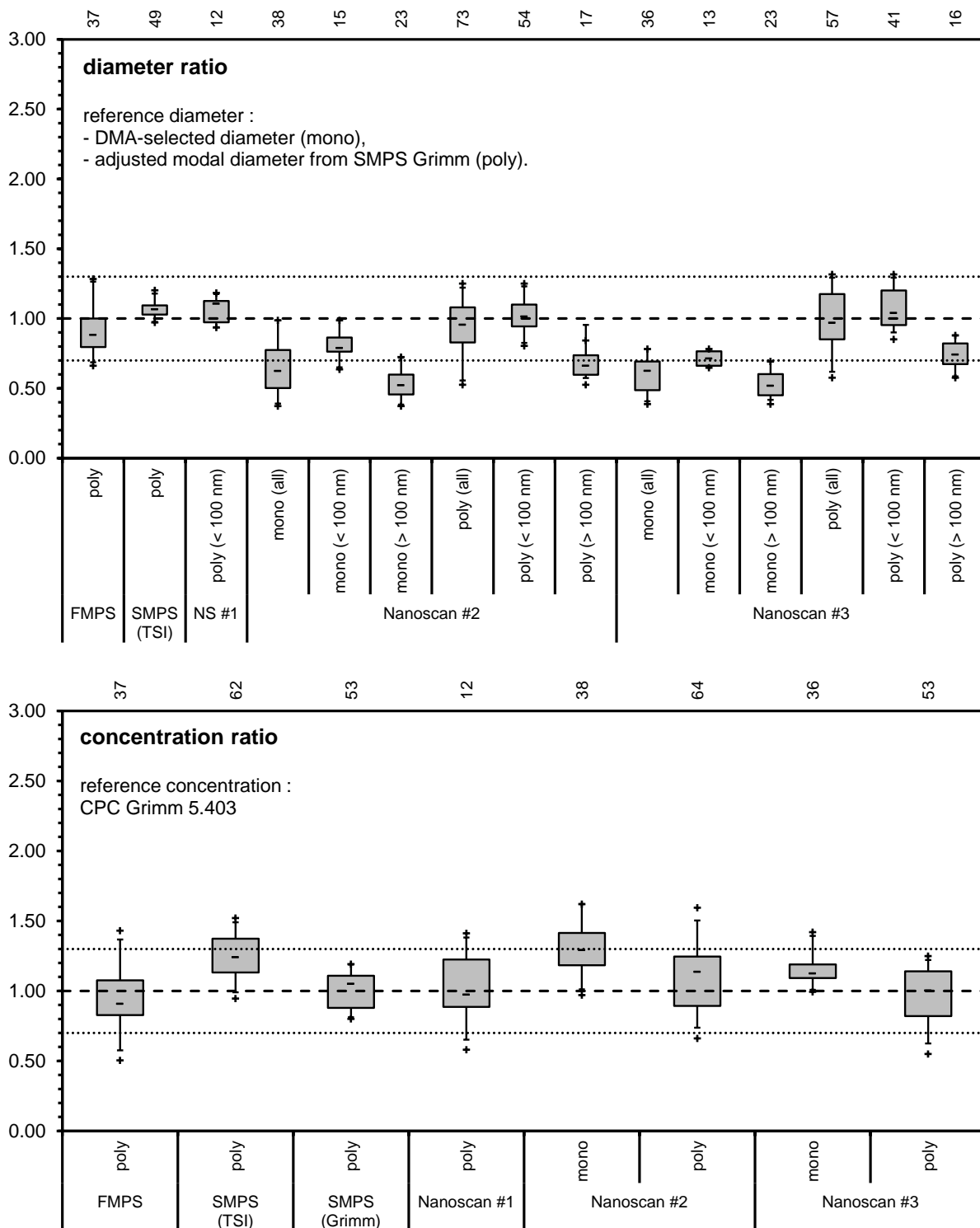
Figure 3. Boxplot of the diameter ratios (top) and number concentration ratios (bottom) found for the electrical mobility spectrometers (NS: Nanoscan).
