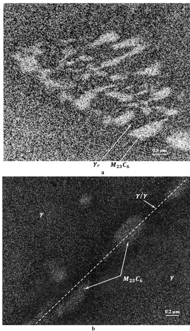
Fig. 9. Chromium depleted area resulting from nucleation and growth of M 23 C 6 rich-chromium carbide after aging at 600 °C during 10 000 h (STEM micrographs): (a) Kα chromium mapping into δ ferrite; (b) Kα chromium mapping of austenite grain boundary region.
