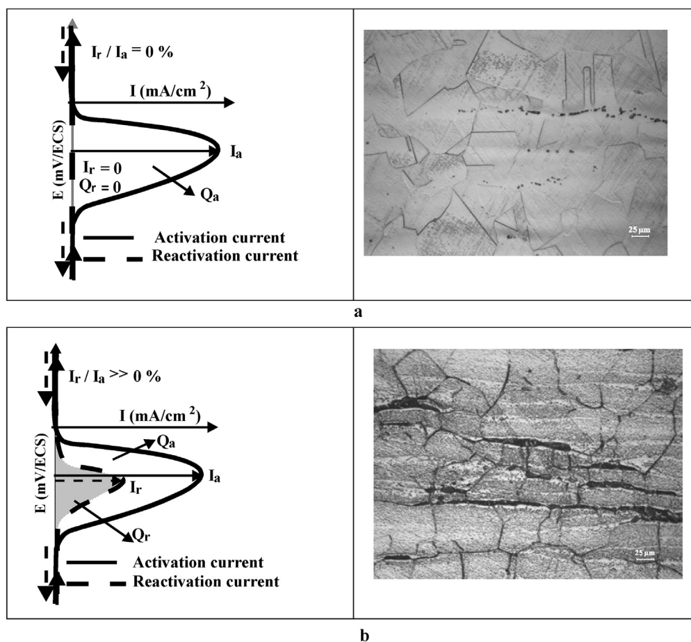
Fig. 1. DL-EPR responses and IGC sensitization criterion: (a) unsensitized material ( I_r/I_a < 1\% ); (b) sensitized material ( I_r/I_a \geq 1\% ).
