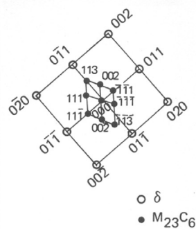
Fig. 4. Decomposition of \delta ferrite after aging at 550 °C during 1000 h (TEM examination): (a) F.K phase (I phase) and M_{23}C_6 carbide at the \delta/\gamma interface; (b) SAD of F.K phase and \delta ferrite matrix; (c) SAD of M_{23}C_6 carbide and \delta ferrite matrix.
