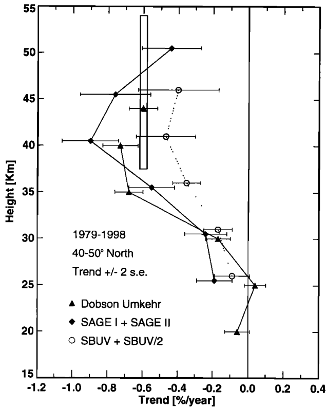
Figure 5. Ozone trends ( \% \text{ yr}^{-1} relative to the mean for the period) at 40^{\circ} - 50^{\circ} N over the period 1979-1998 calculated from the following measurement systems: Three Dobson Umkehr stations (Arosa, Boulder, and Haute Provence) reported at individual layers 4 through 8 (triangles) and layers 8+9+10 (plotted as a vertical bar from \sim 37 to 54 km with triangle); SAGE I/II average sunrise and sunset observations (diamonds) reported at individual layers 4-10; SBUV+SBUV/2 weekly averages (circles) reported at individual layers 5 through 9. All error bars are 95% confidence intervals of the trend and represent statistical uncertainty only. Small vertical offsets are for clarity only (e.g., all values plotted near 30 km represent layer 6 results).
