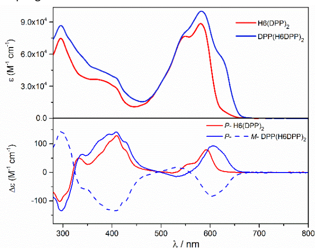
Figure 7. UV-vis (top) and ECD (bottom) spectra of H6(DPP) 2 (red) and DPP(H6DPP) 2 (blue) in dichloromethane solution at 298 K ( \sim 10^{-5} M).
