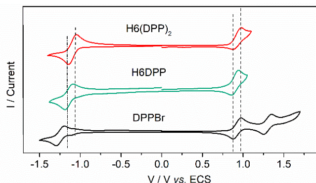
Figure 5. Cyclic voltammograms of DPPBr , H6DPP and H6(DPP) 2 versus saturated calomel electrode (SCE) as the reference and 0.1 M Bu 4 NPF 6 in dichloromethane as the electrolyte.
