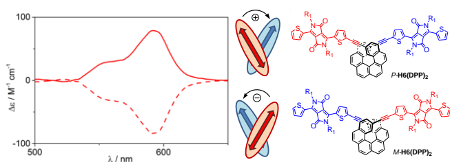
Figure 6. Relation between the helical arrangement of the dpp units around the P - or M -helicenic core and the respective positive or negative exciton coupling signature.
