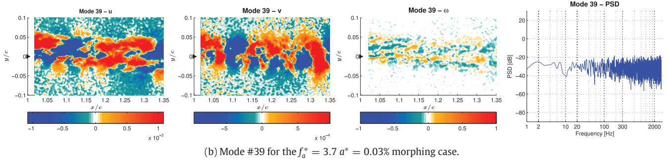
Fig. 22. Comparison of two POD modes. From left to right: stream-wise velocity component; crossflow velocity component; vorticity of the corresponding mode; PSD of the temporal coefficients of each POD mode.
