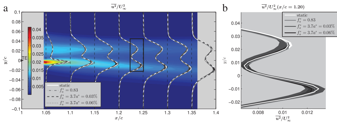
Fig. 10. Time average of the squared stream-wise perturbation velocity \bar{u}^2 for the static case and profiles for the non-actuated and the actuated configurations; Re = 0.5 \cdot 10^6 . The thicknesses of the envelopes corresponds to minimum and maximum values calculated using the three acquisitions.
