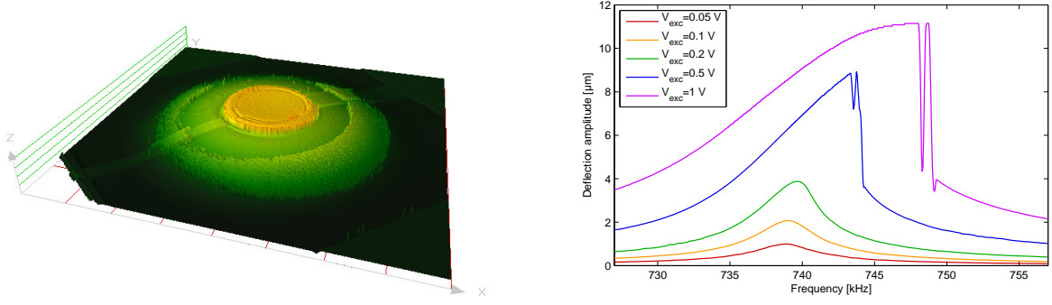
Figure 2. Static non-planar geometry of a membrane and dynamic non-linear behaviour. Experimental results.
