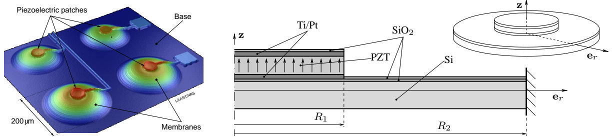
Figure 1. A 2 \times 2 resonant membranes matrix biosensor. Cross section of a layered membrane.
