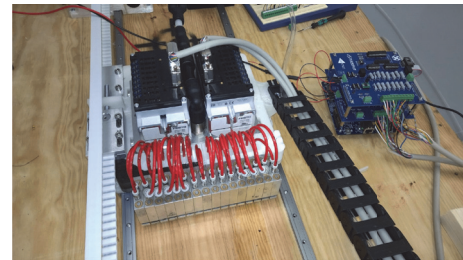
FIGURE 13: IED control system for the head (pneumatic valve actuator terminal).
