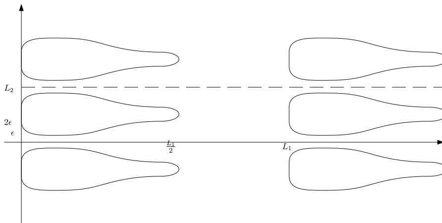
Figure 3: The periodic domain \Omega_3
